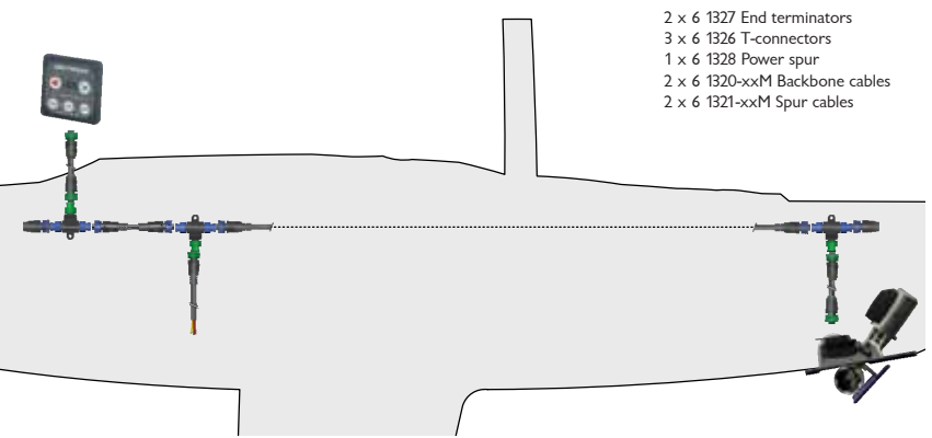
Example of the control wiring with S-link system for boats with one control position and one retractable thruster
