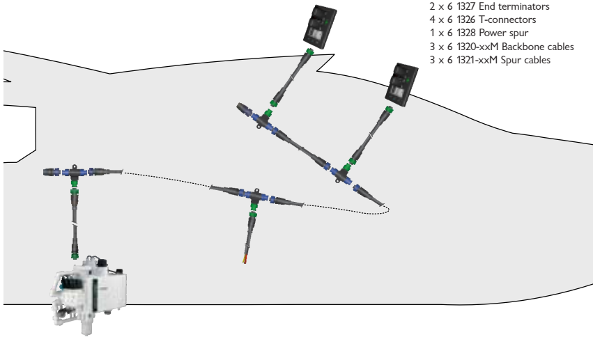
Example of the control wiring with S-link system for boats with two control positions and hydraulic thruster system
